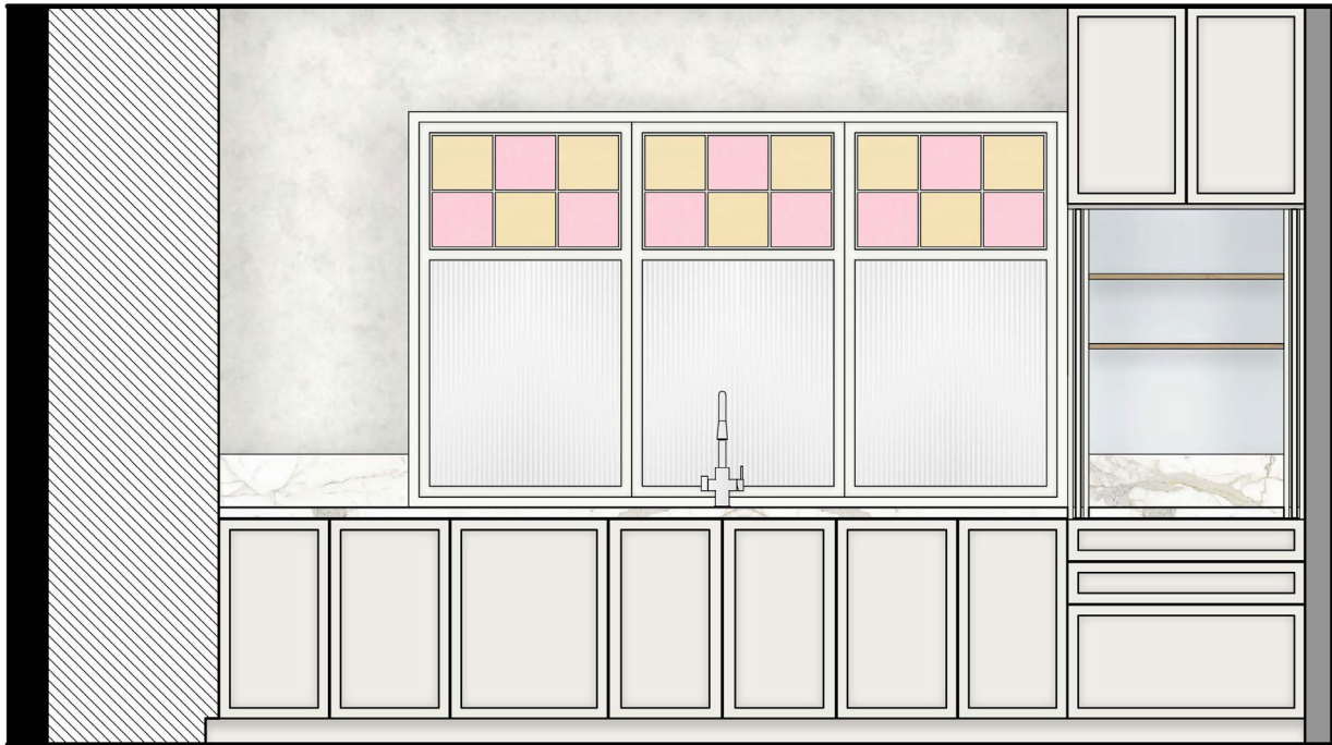
1 KITCHEN - ELEVATION B SCALE: 1:20
